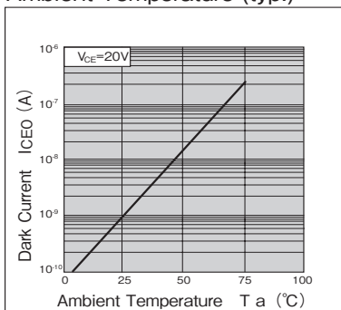
Dark Current vs. Ambient Temperature (typ.)
