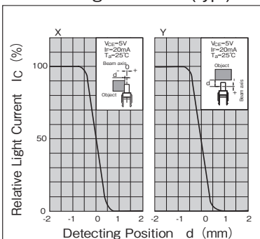
Detecting Position vs. Relative Light Current (typ.)
