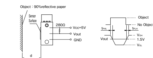
※3:Measuring circuit of Response time
