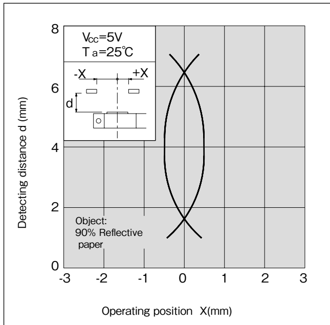
Operating Position vs Detecting Distance 2 (typ.)
